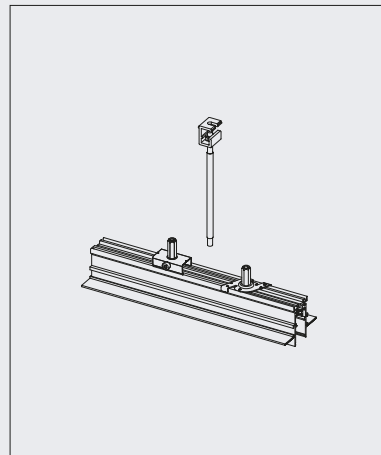
Trimless tracks
