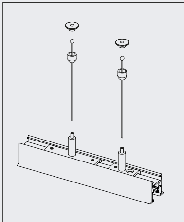
Recessed track
