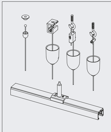
Ceiling/Suspended track
