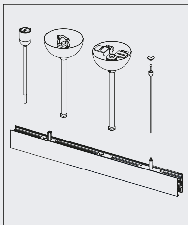
Double tracks
